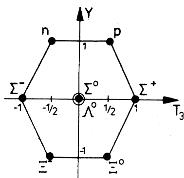
1. ábra: A J^\pi = \frac{1}{2}^+ barionok.
